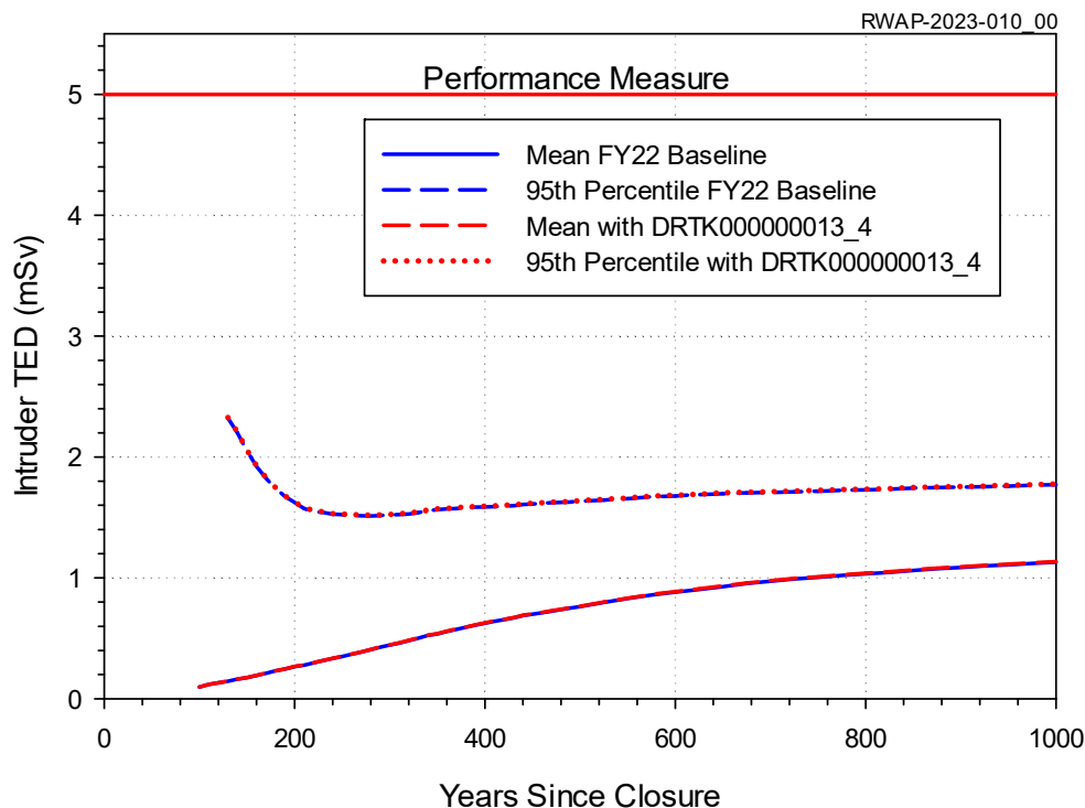
Figure 3. Acute Construction Intrusion Scenario TED Time History with and without the DRTK000000013_4 Waste Stream
