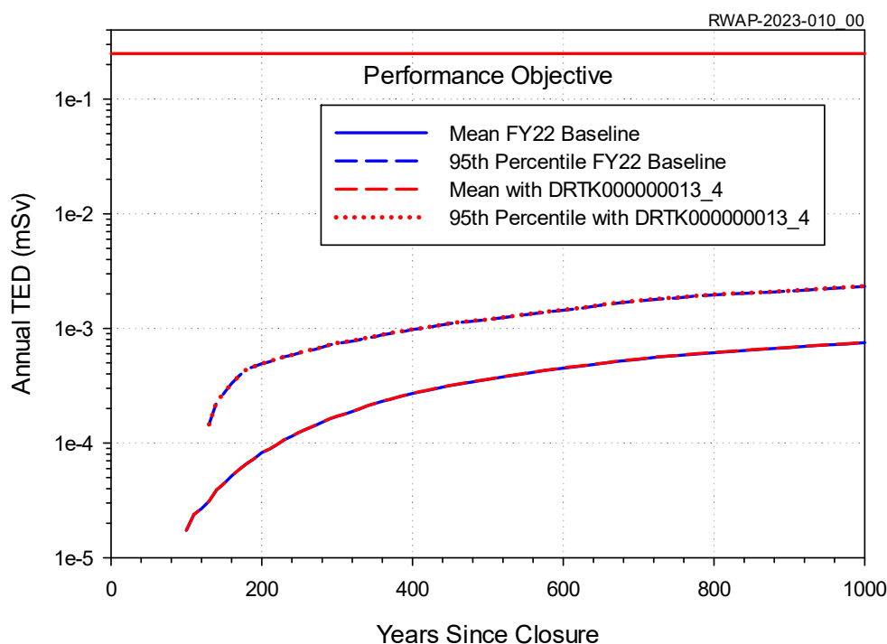
Figure 2. All-Pathways Annual TED Time History for a Resident at the 100-m Boundary with and without DRTK000000013_4 Waste Stream
