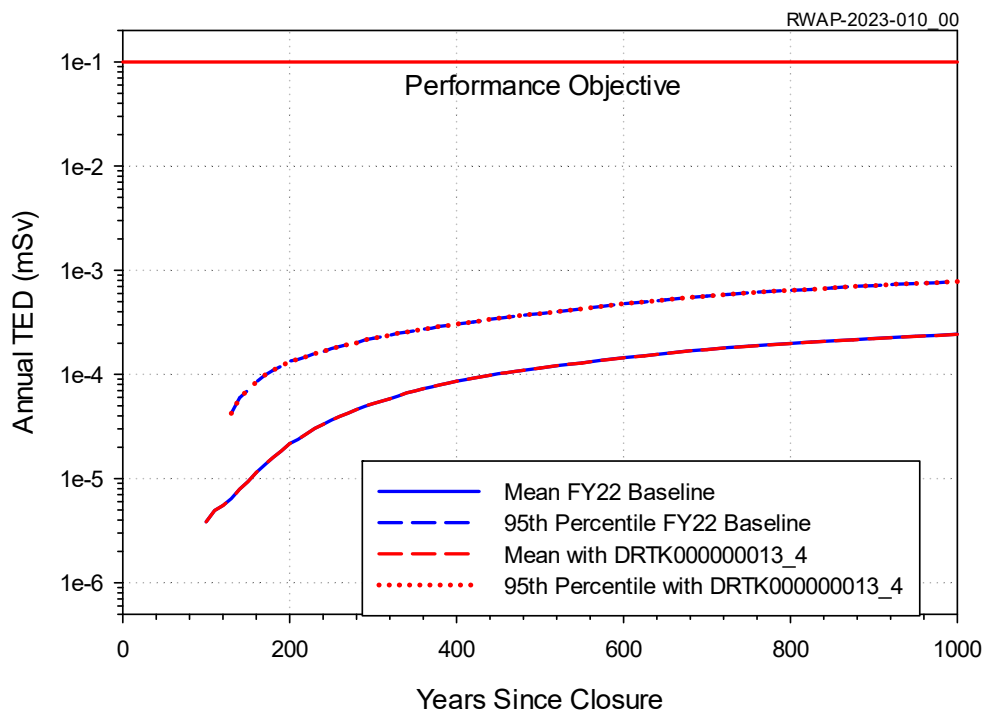
Figure 1. Air Pathway Annual TED Time History for a Resident at the 100-m Boundary with and without the DRTK00000013_4 Waste Stream
