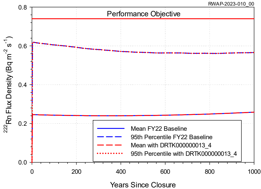
Figure 4. 222 Rn Flux Density Time History with and without the DRTK00000013_4 Waste Stream
